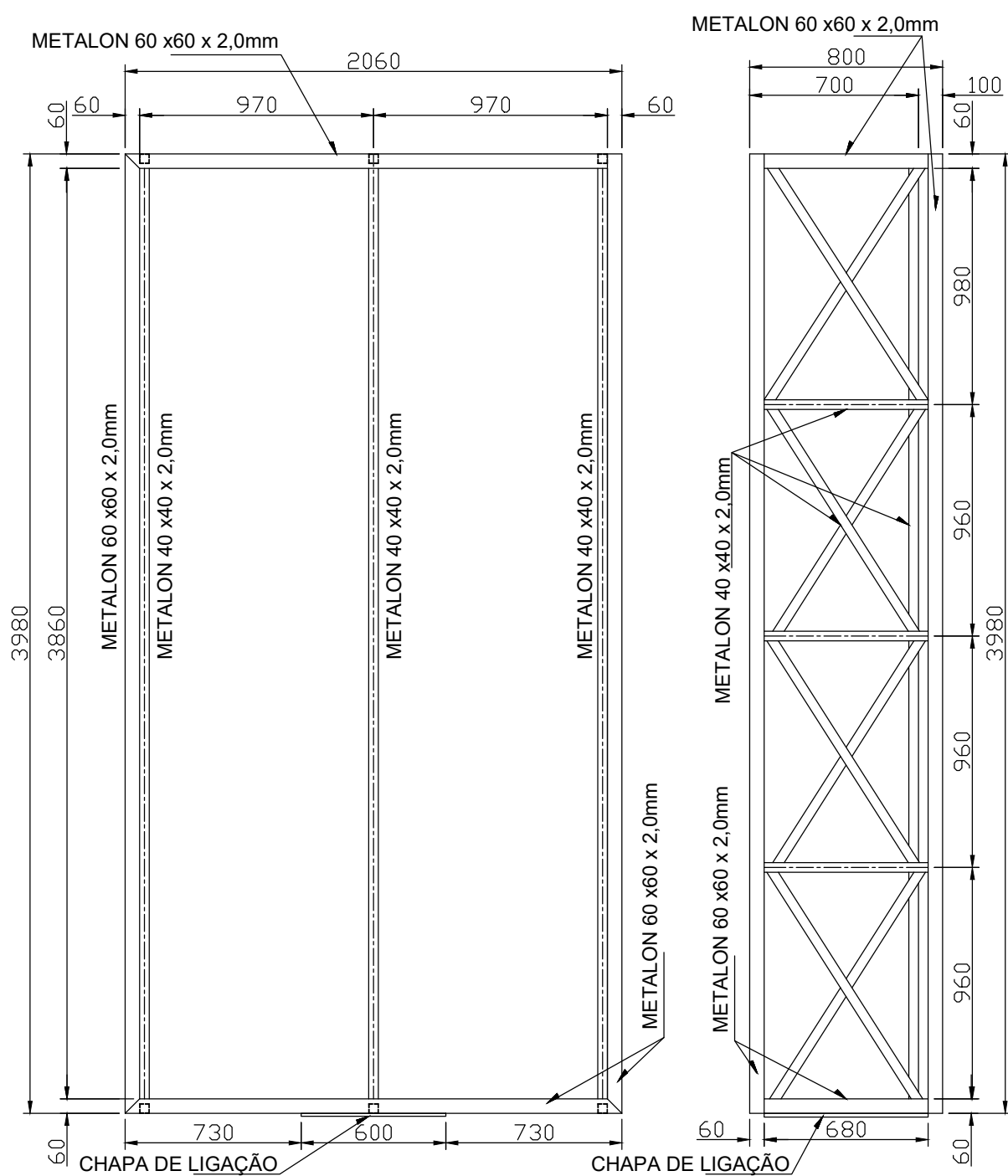
VISTA FRONTAL
